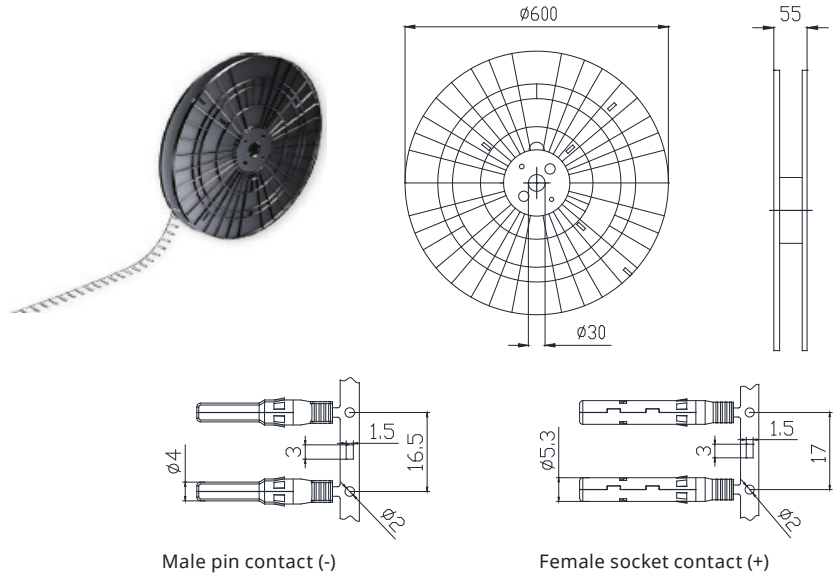
Male pin contact (-)
