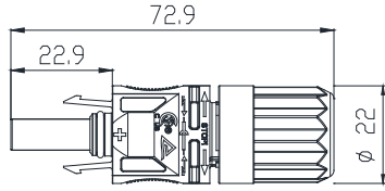
Female connector (+)
