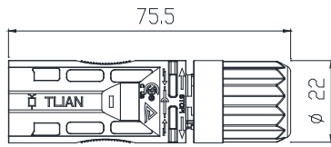
Male connector (-)
