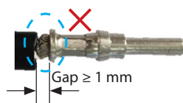
Incorrect crimping
