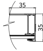
Frame Cross Section A-A
